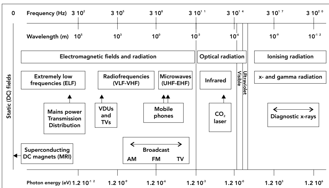
Electromagnetic spectrum
